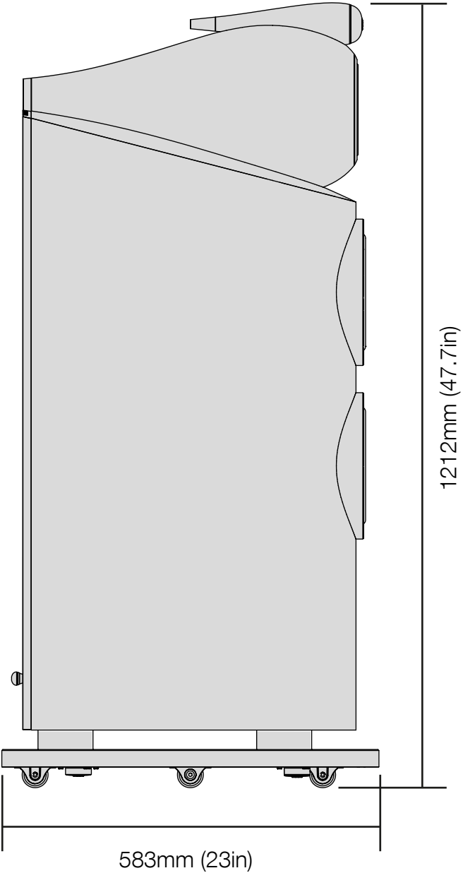
SIDE
