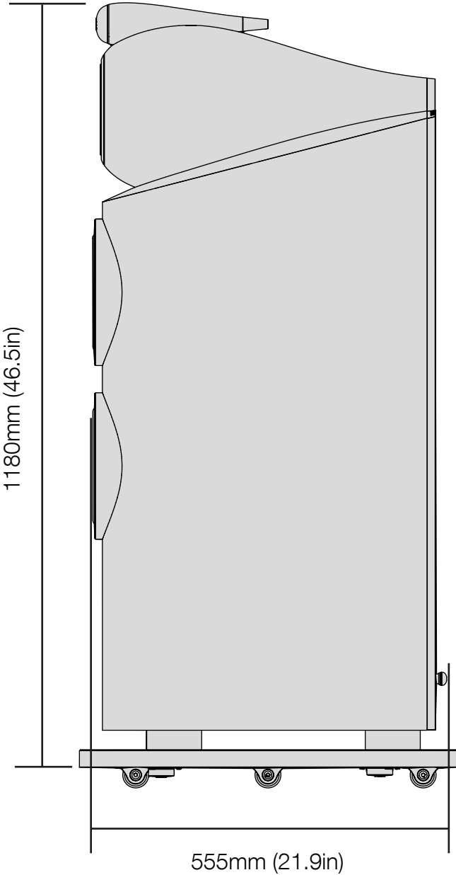
SIDE
